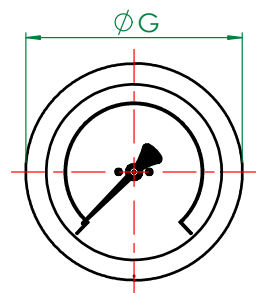
MODEL - 632-BC Direct Mounted - Rear Connect
