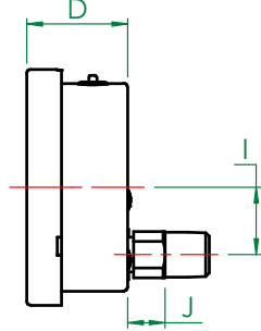
MODEL - 632-BC Direct Mounted - Rear Connect
