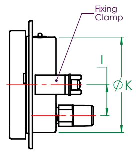
MODEL - 634 Flush Mounted - Clamp Fixing
