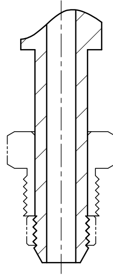
COMPLETED MEDIUM PRESSURE CONNECTION
