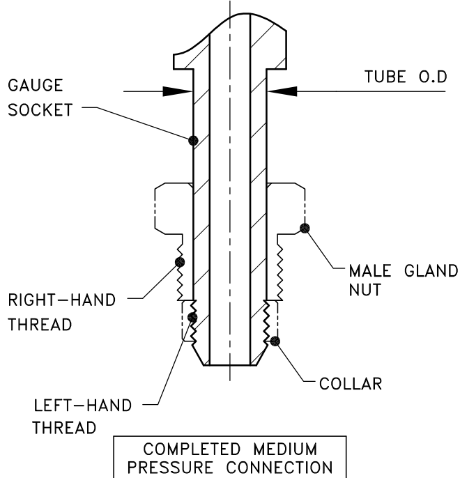
COMPLETED MEDIUM PRESSURE CONNECTION
