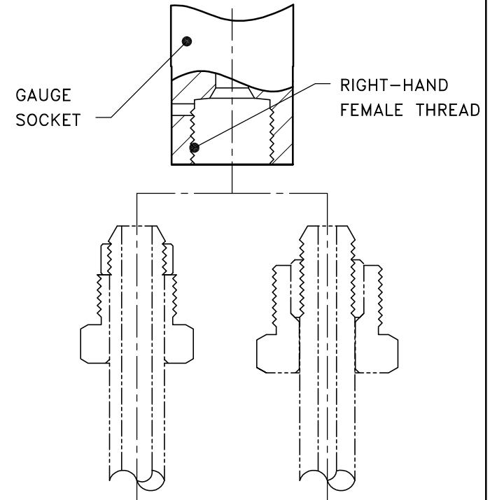
COMPLETED HIGH PRESSURE CONNECTION
