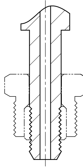
COMPLETED HIGH PRESSURE CONNECTION
